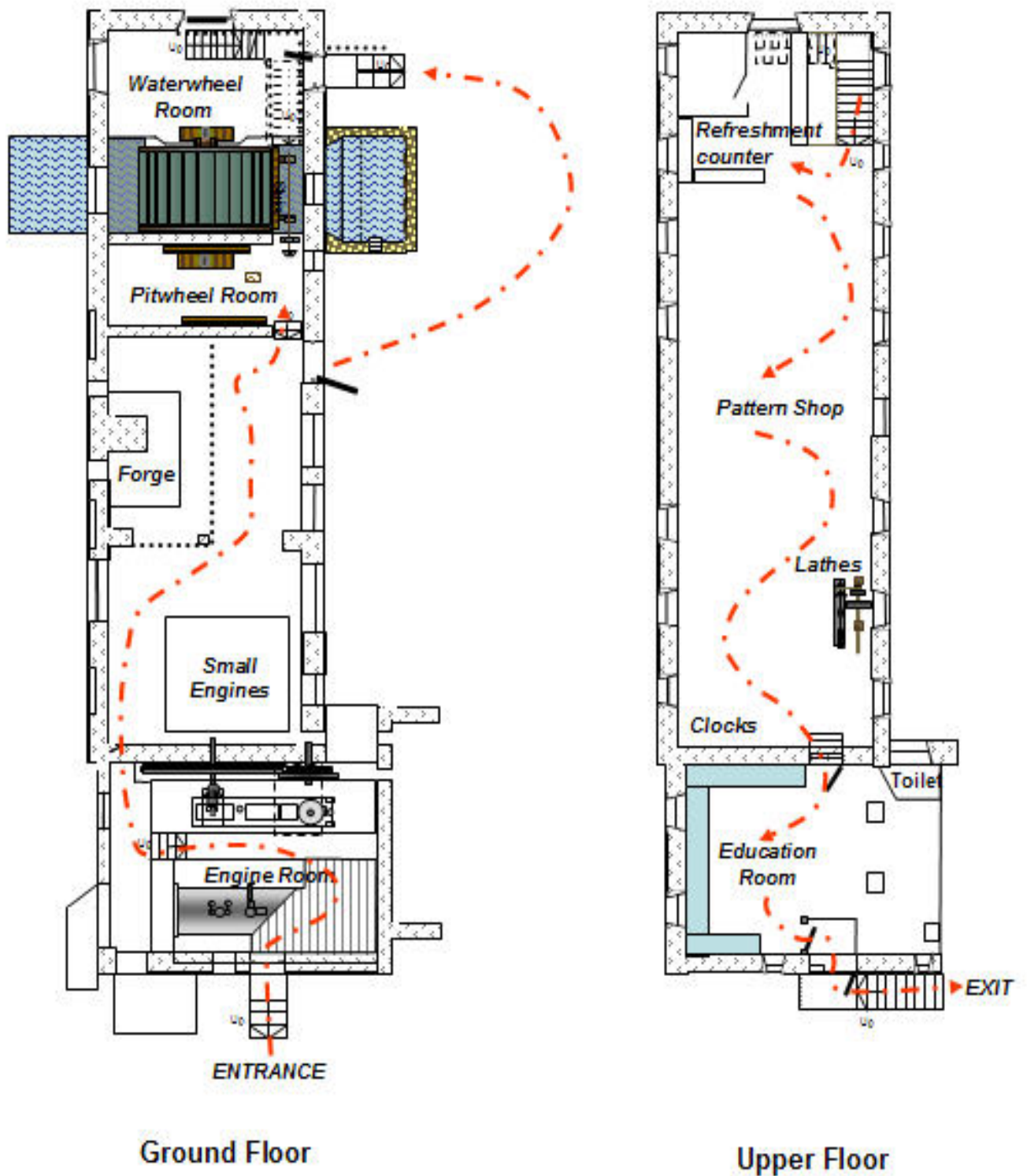
Figure 1 Combe Mill Floor Plans
